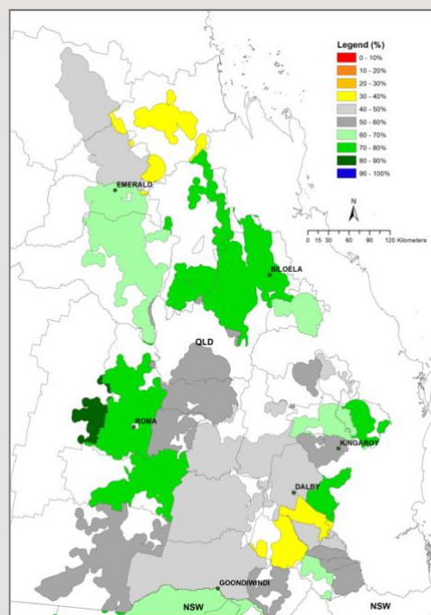
Map 2: Aggregated soil water recharge status (%) as at 1st May 2020. Short summer fallow simulated
